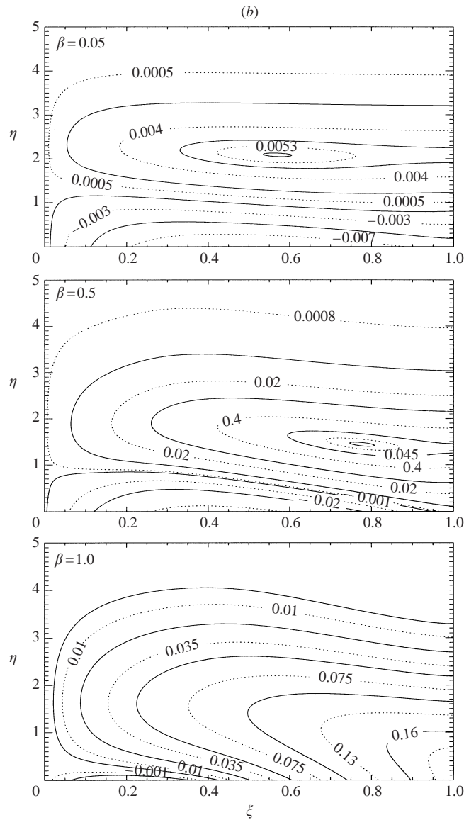
FIGURE 14. Rectangular corner configuration, upper solution branch in region (iii): (a) evolution of u(\eta, \xi) profiles, \beta and \xi as indicated. (b) streamwise vorticity \omega(\eta, \xi) contours, \beta as indicated.
