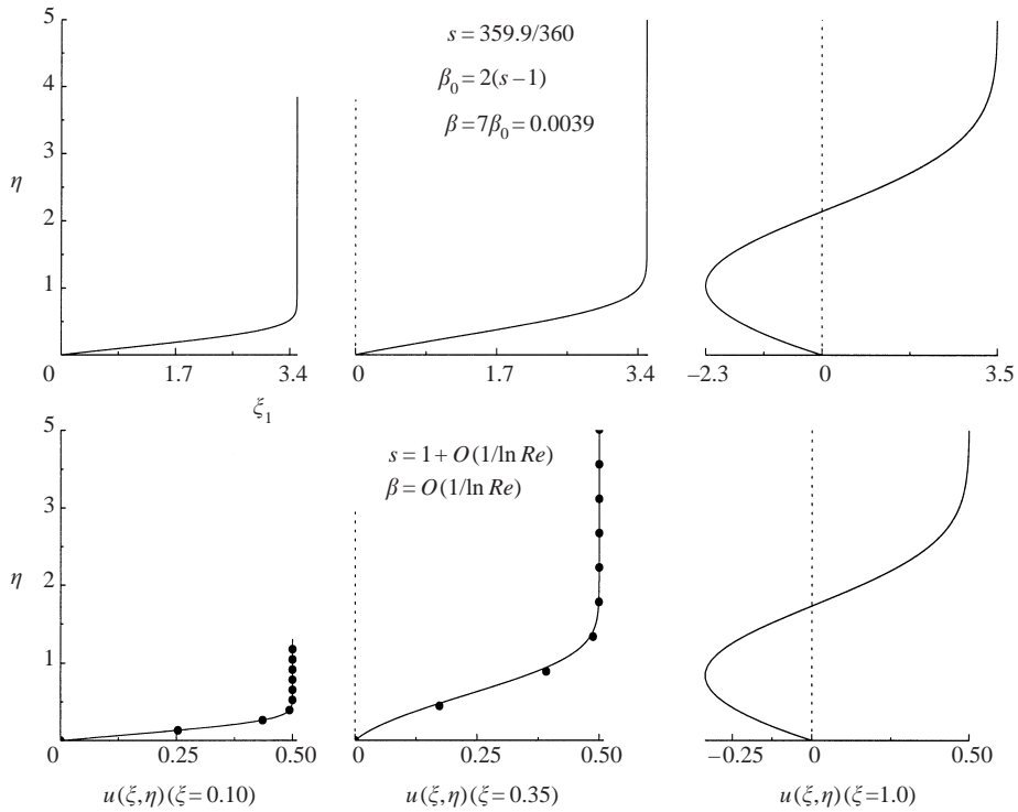
FIGURE 20. 359.9°-convex corner and quarter-infinite flat plate limit s \rightarrow 1 , region (iii): u(\xi, \eta) profiles, \beta and \xi as indicated; ●, series expansions (7.11) solutions.
