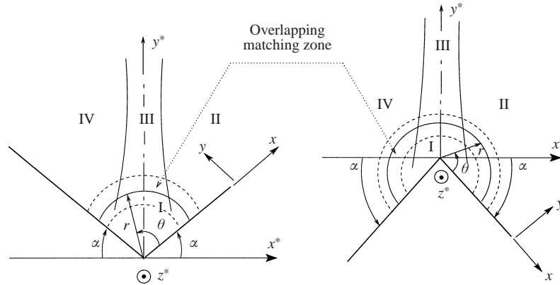
FIGURE 2. A cross-section showing potential flow structure in the vicinity of the corner.
