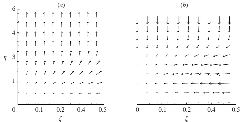
FIGURE 8. Almost planar corners, region (i), K = 0 : secondary flow vector plots. (a) \beta = 0 . (b) \beta = 1.0 .
